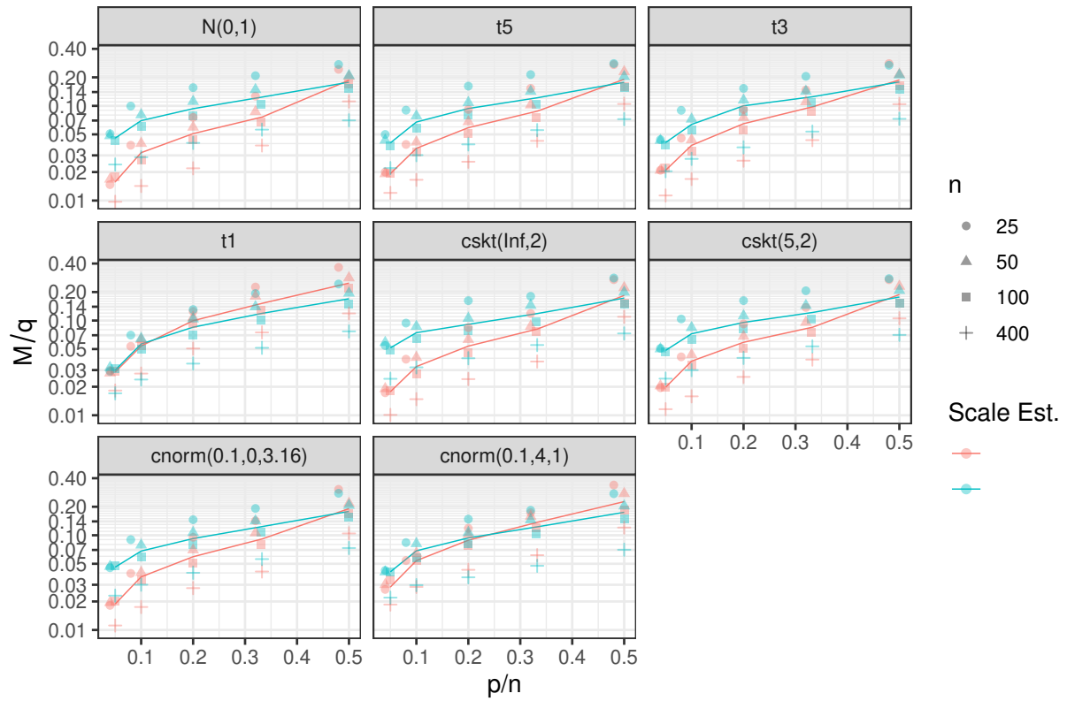
Figure 9: M/q statistic for bisquare \psi .
