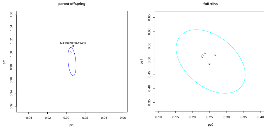
Figure 2: Observed pairs with prediction ellipses for parent-offspring pairs (left panel) and full siblings (right panel) superposed.
